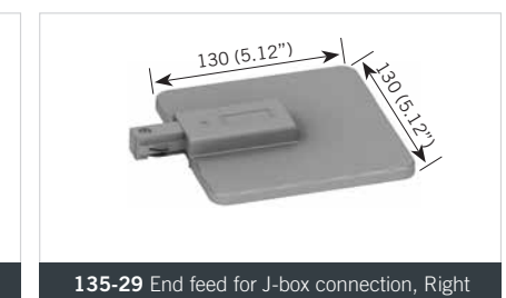
135-29 End feed for J-box connection, Right
