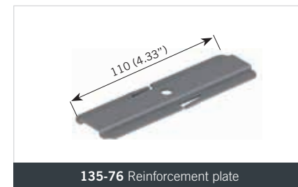
135-76 Reinforcement plate
